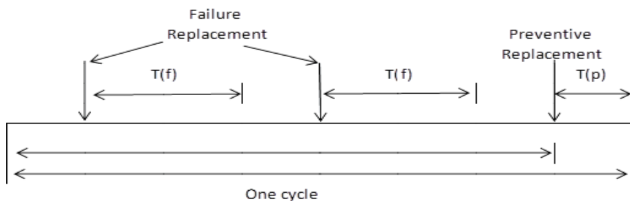
Figure 2: Downtime minimization: optimal interval.
